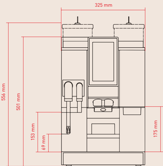
Schaerer Coffee Club Depth: 570 mm
