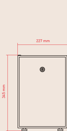
Side cooling unit left Depth: 469 mm
